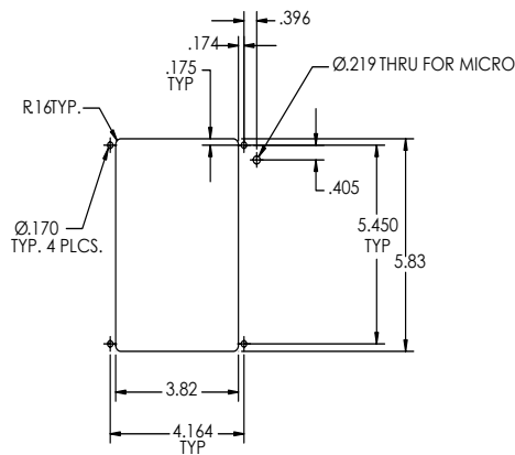
MOUNTING HOLE SPECIFICATIONS
