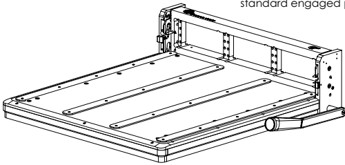
310104334 & 310104385: G12/G12x receiver with a 20" platform show with handle in the standard engaged position.
