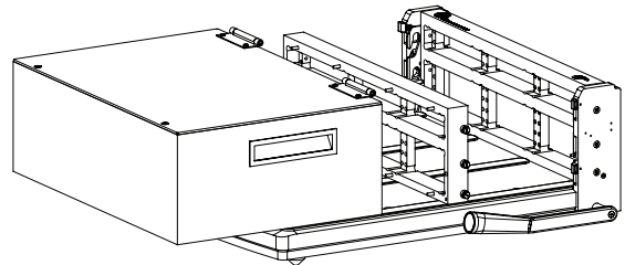
G12x Enclosure (Part # 410 104 474)
