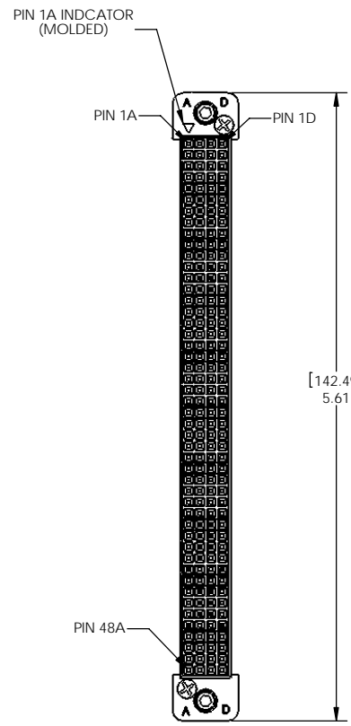
VIEW OF VPC RECEIVER MODULE FRONT MATING (ITA) SIDE P/N 510150130
