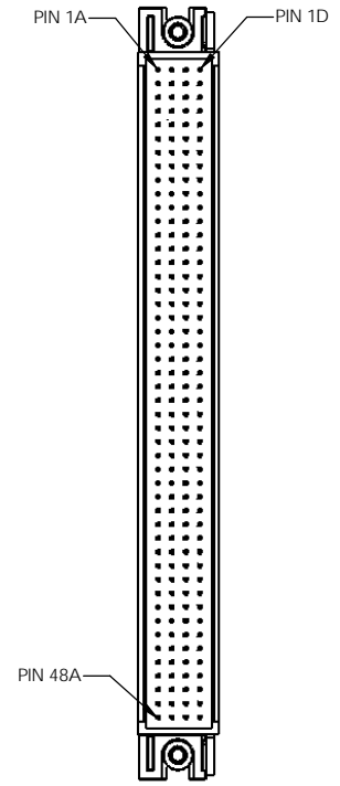
SECTION A-A SCALE 1.3 : 1 VIEW OF BOARD MOUNTED RIGHT ANGLE HEADER MATING SIDE
