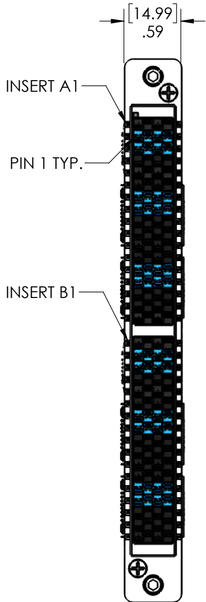
34 POSITION SIM RECEIVER MODULE MATING FACE
