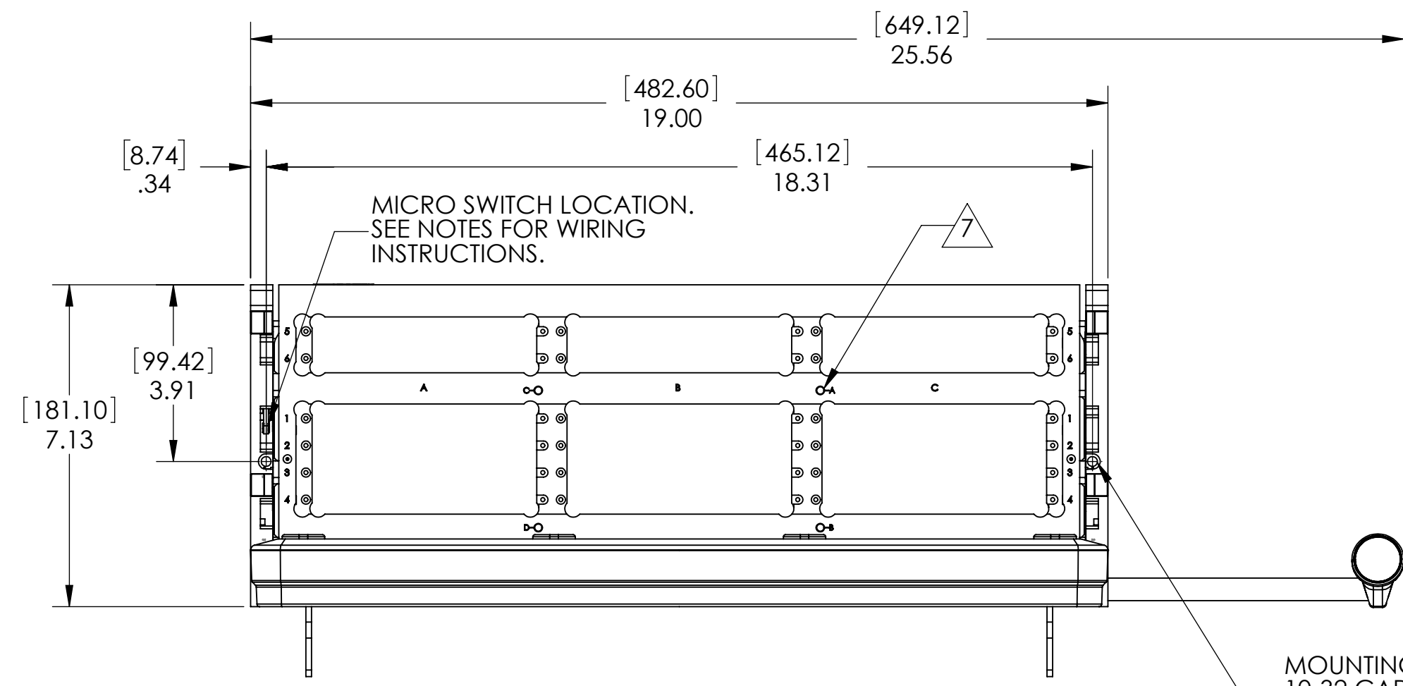
DETAIL A SCALE 2 : 3
