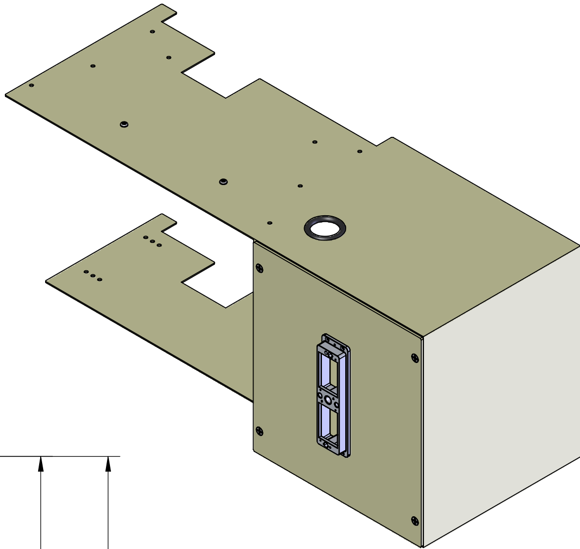
ICON RECEIVER (P/N 310104101) SHOWN FOR REFERENCE ONLY.
