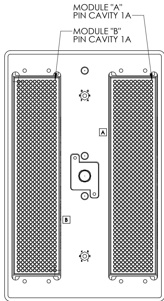
CONNECTOR MATING VIEW
