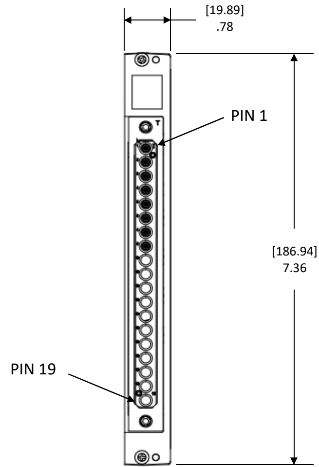
J1 MATING FACE
