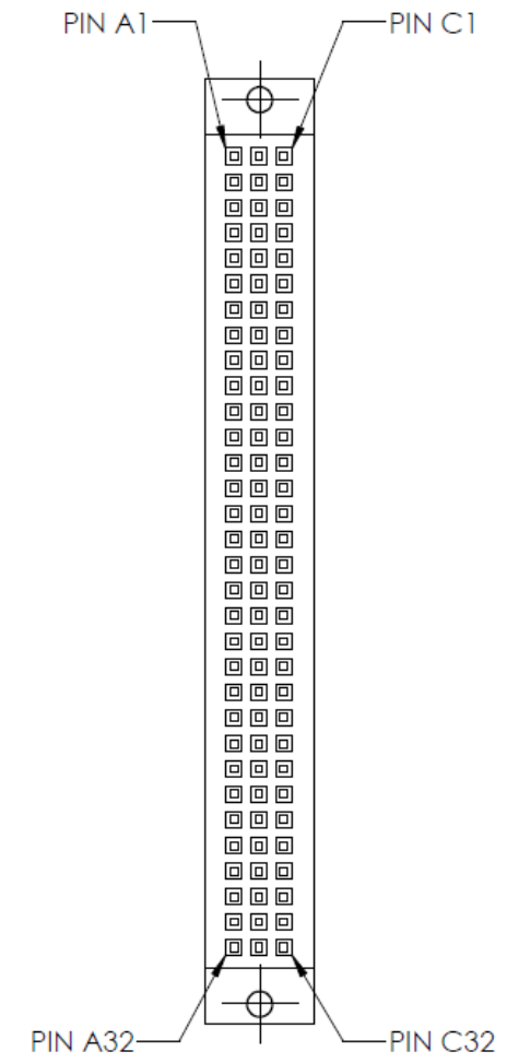
96 PIN FEMALE DIN MATING FACE J1
