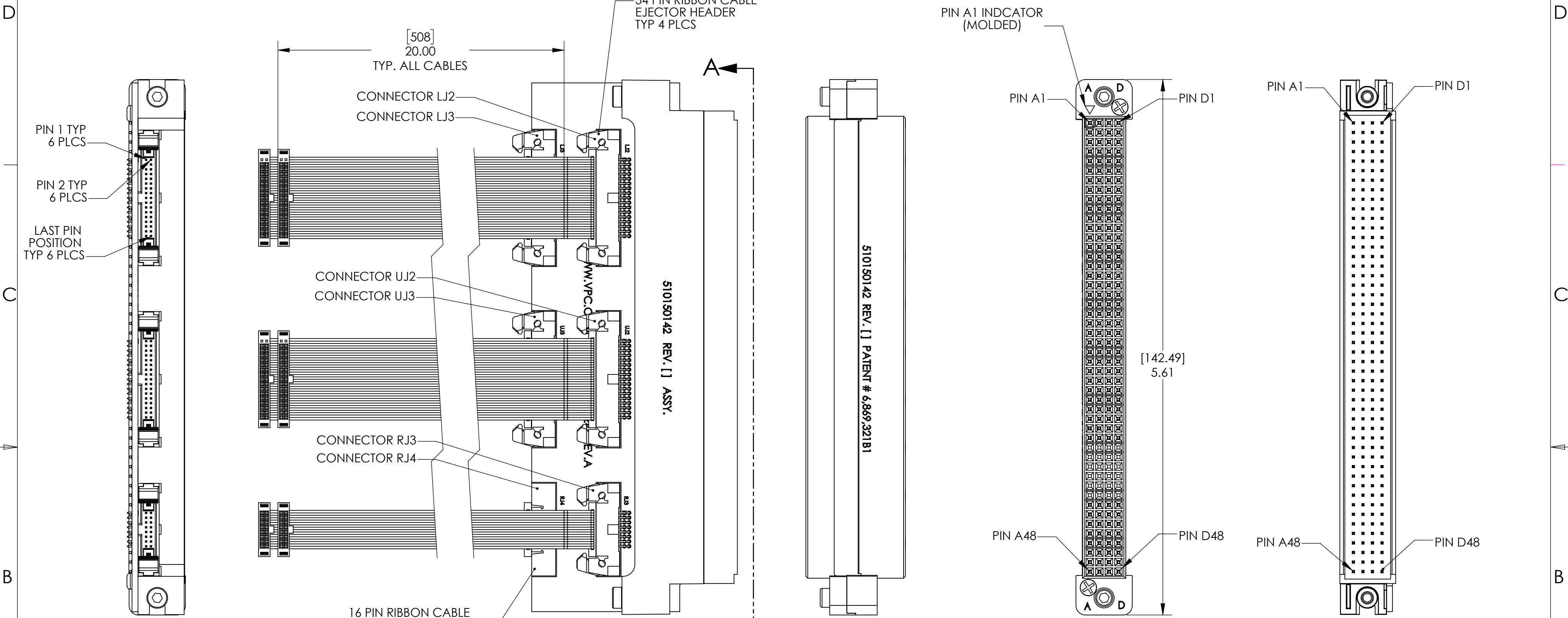
VIEW OF RIBBON CABLE CONNECTOR MATING SIDE
