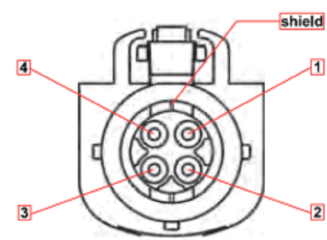
ROSENBERGER HSD P/N D4K10A-1D5A5-Z MATING FACE
