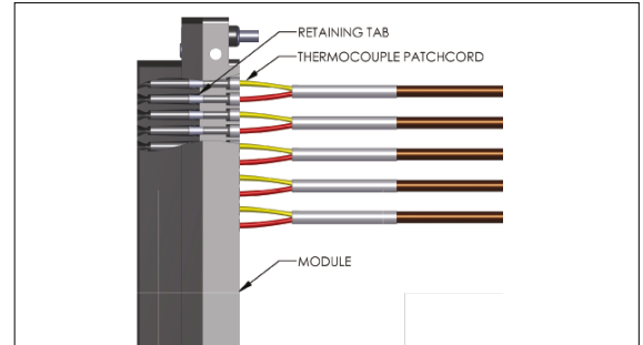
Figure A. Contacts inserted into the module.
