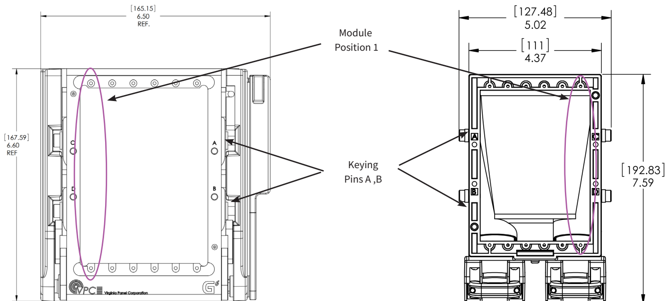
Figure A. G6 Receiver front/mating face
