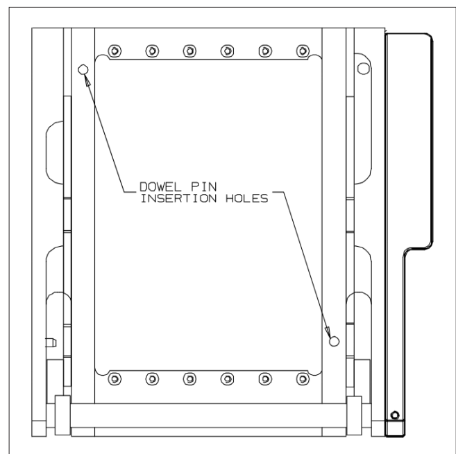
Figure B. Front side of receiver.
