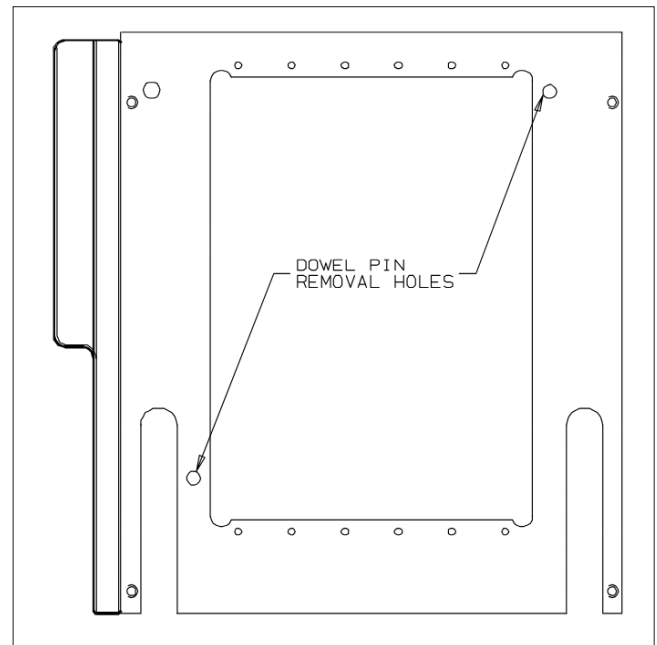
Figure A. Back side of receiver
