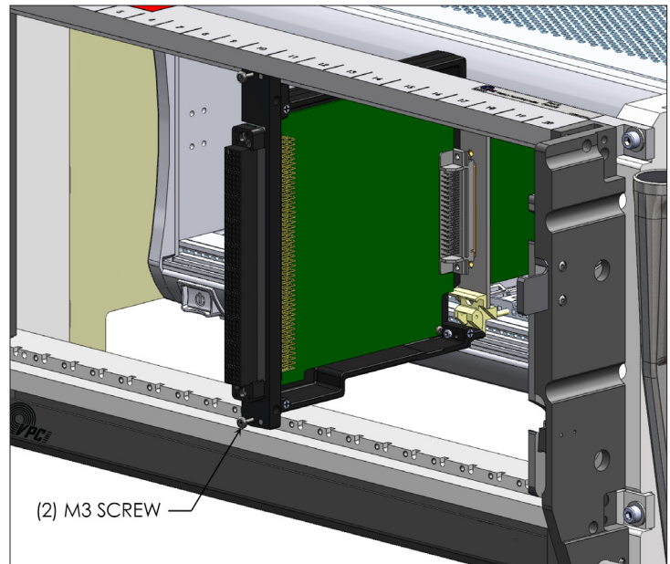
Figure A. Secure adapter to the receiver frame
