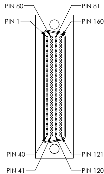
160 PIN CONNECTOR MATING VIEW
