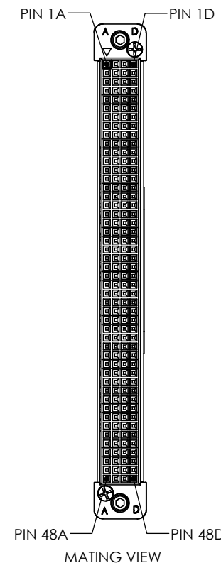
MATING VIEW
