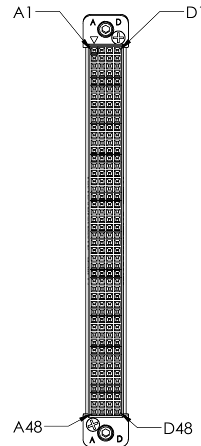
P1 MATING FACE
